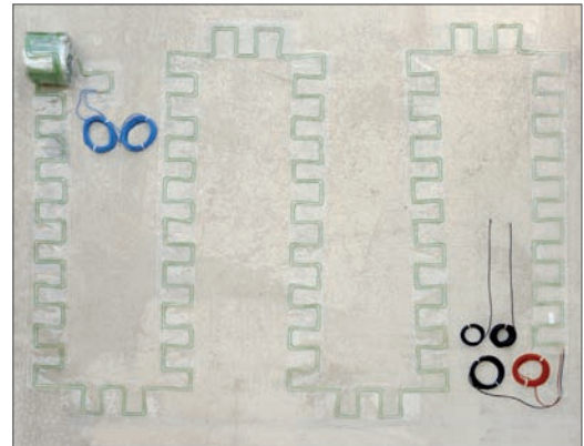
Example installation: approved design with spare heating cable and temperature sensors
